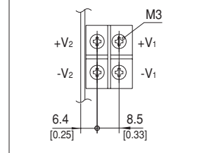
Terminal in detail (Module S, T, U)
