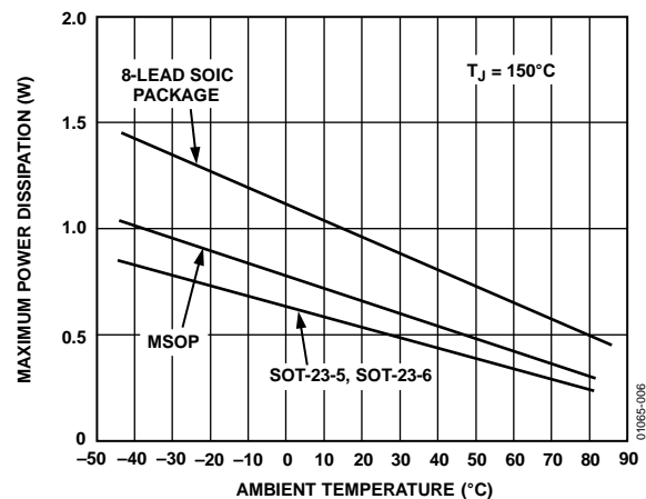
Figure 6. Maximum Power Dissipation vs. Temperature for AD8061/AD8062/AD8063
