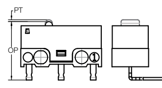
OP FROM TERMINAL (FOR TYPE 50 & 60 TERMINAL)
