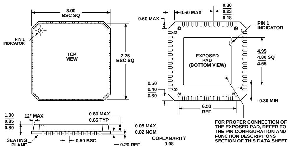
COMPLIANT TO JEDEC STANDARDS MO-220-VLLD-2 Figure 78. 56-Lead Lead Frame Chip Scale Package [LFCSP_VQ] 8 mm × 8 mm Body, Very Thin Quad (CP-56-3) Dimensions shown in millimeters
