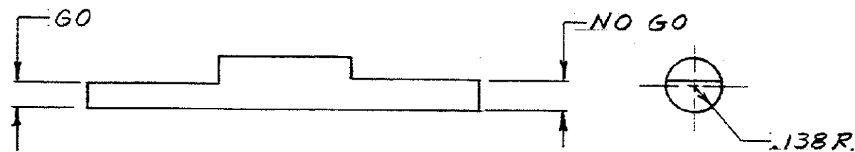
SUGGESTED PLUG GAGE DESIGN
