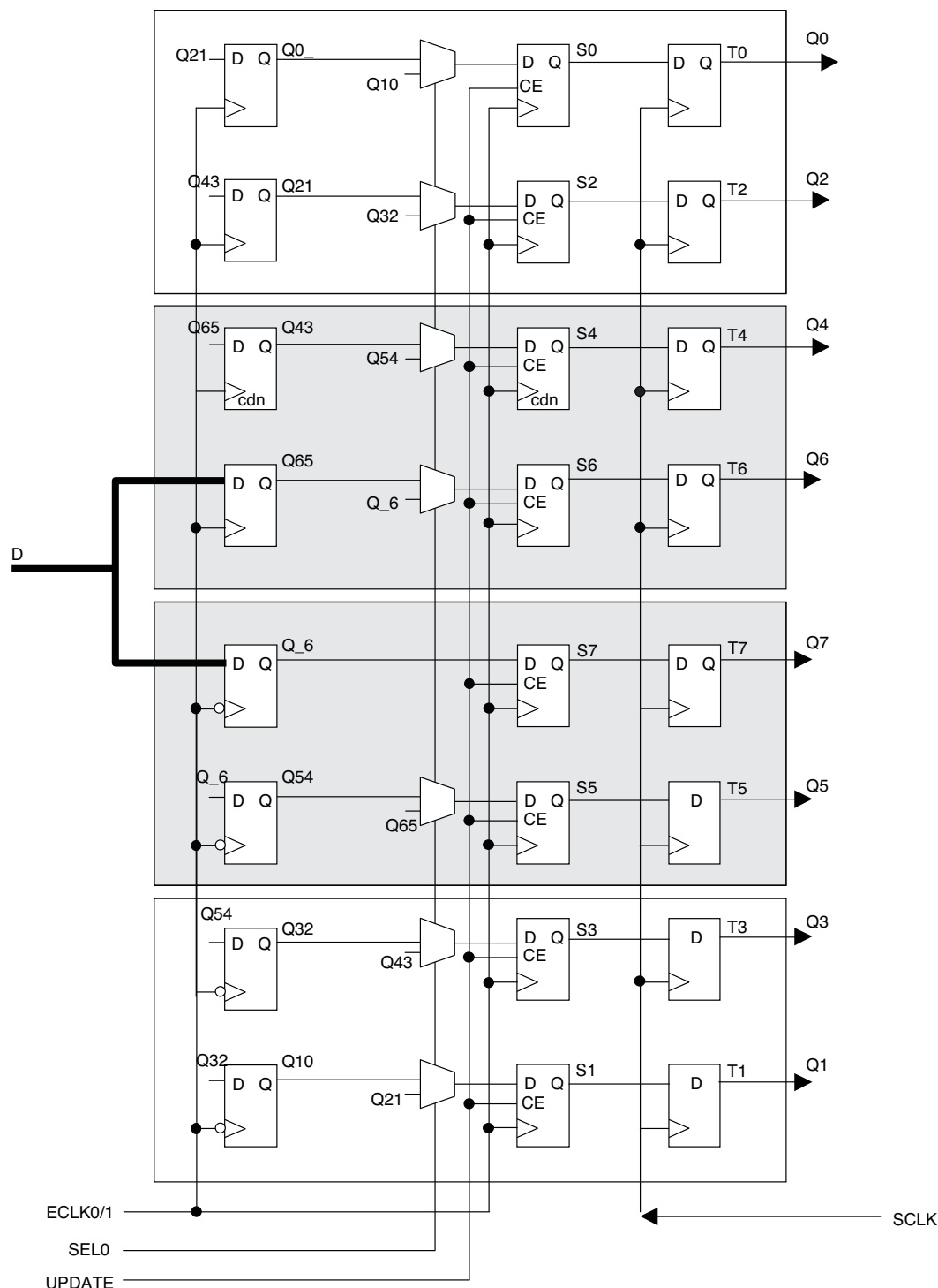
Figure 2-16. Input Gearbox
