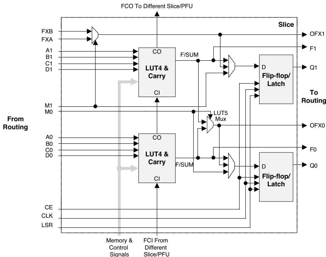
Figure 2-4. Slice Diagram
