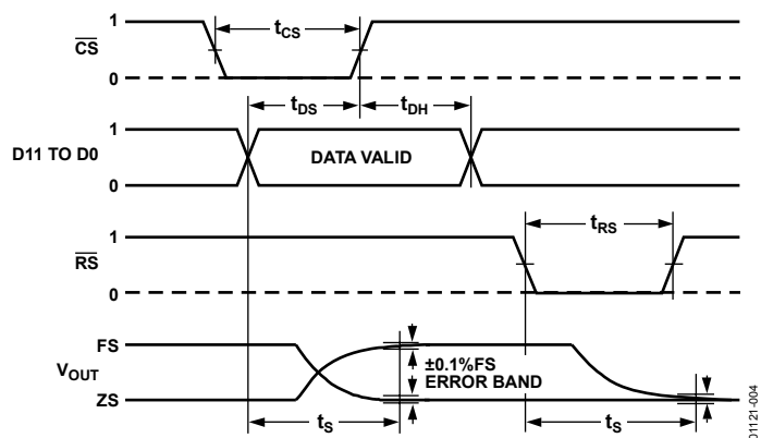
Figure 2. Timing Diagram
