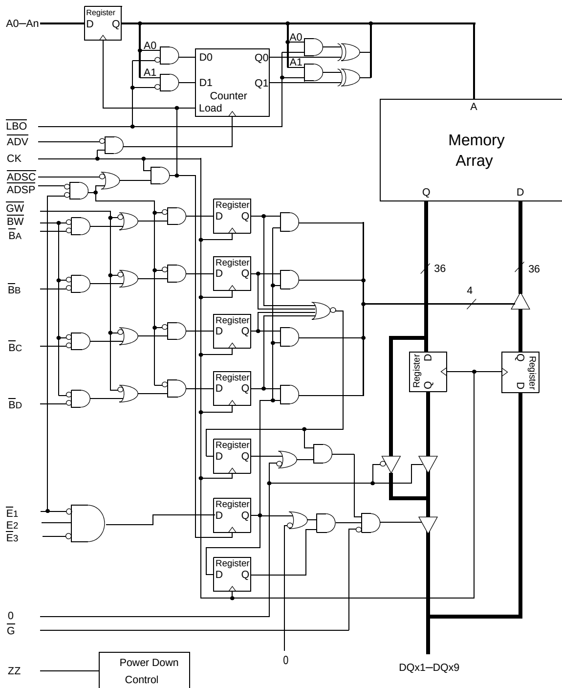
GS8160F18/32/36D Block Diagram
