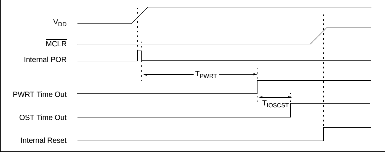
FIGURE 14-4: TIME-OUT SEQUENCE ON POWER-UP (DELAYED MCLR): CASE 2
