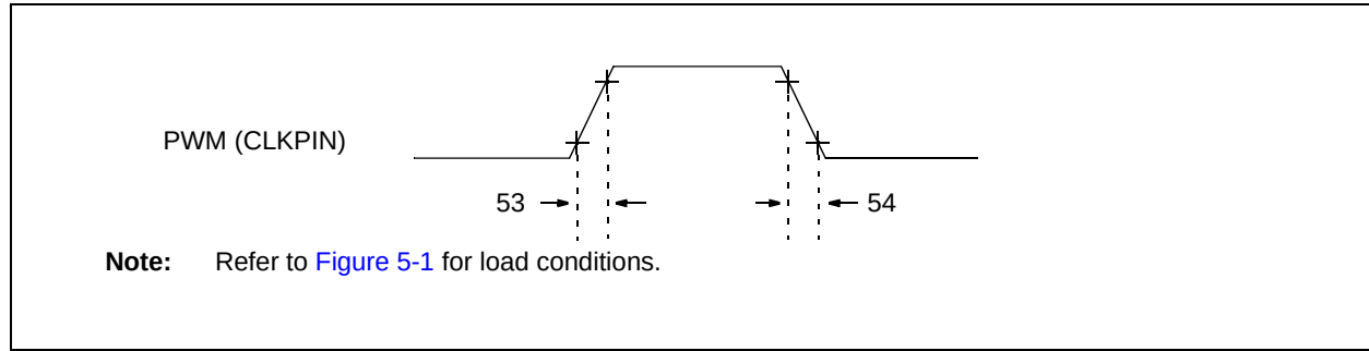
FIGURE 5-6: PWM TIMING
