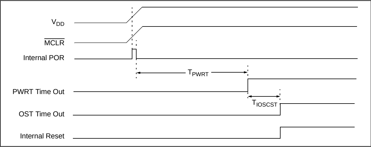
FIGURE 14-5: TIME-OUT SEQUENCE ON POWER-UP (MCLR WITH V DD )
