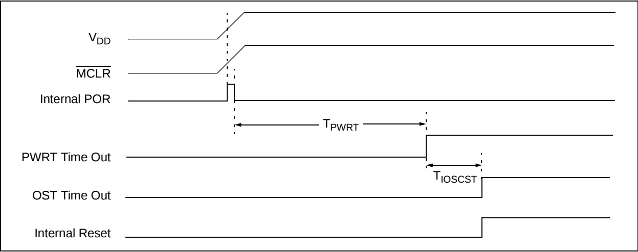
FIGURE 14-5: TIME-OUT SEQUENCE ON POWER-UP (MCLR WITH VDD)
