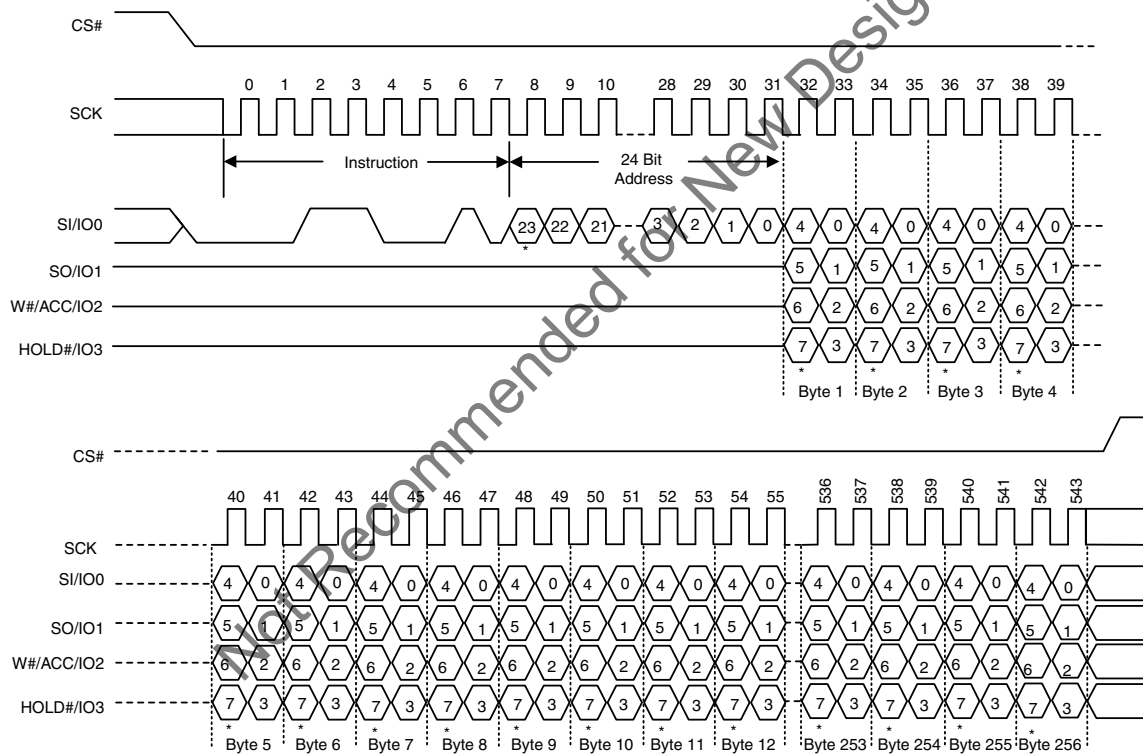
Figure 27. QUAD Page Program Instruction Sequence
