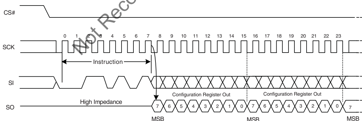
Figure 23. Read Configuration Register (RCR) Instruction Sequence
