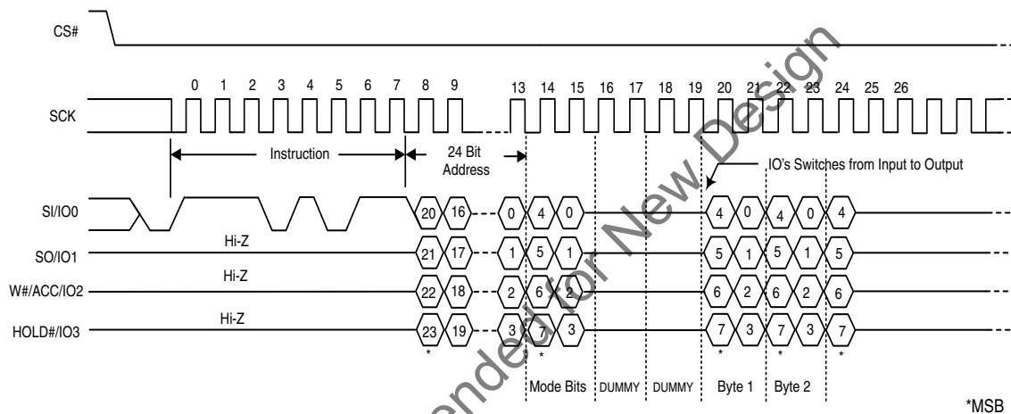
Figure 16. QUAD I/O High Performance Instruction Sequence
