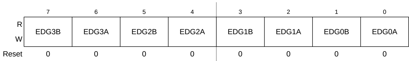
Figure 16-17. Timer Control Register 4 (TCTL4)
