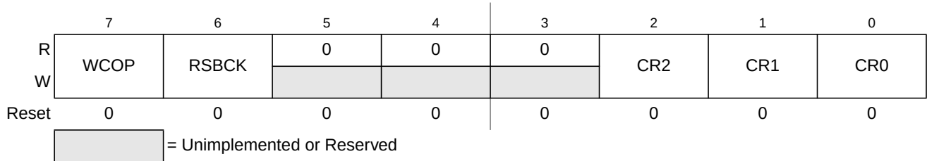
Figure 5-12. CRG COP Control Register (COPCTL)
