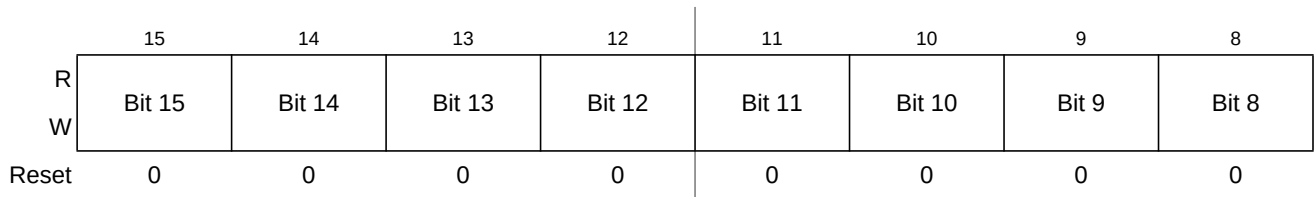
Figure 19-17. Debug Comparator A Register High (DBGCAH)
