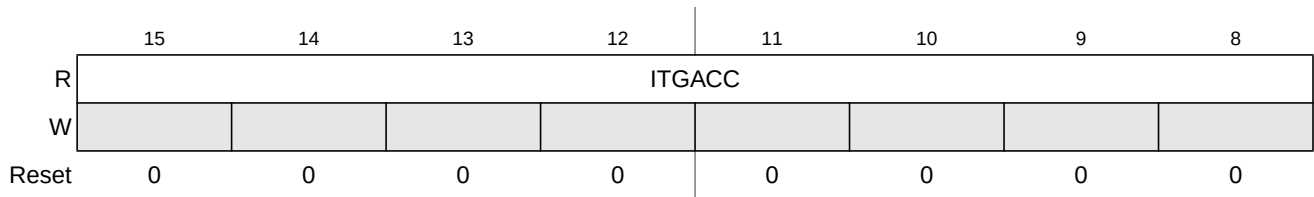
Figure 10-8. Integration Accumulator Register High (ITGACC)
