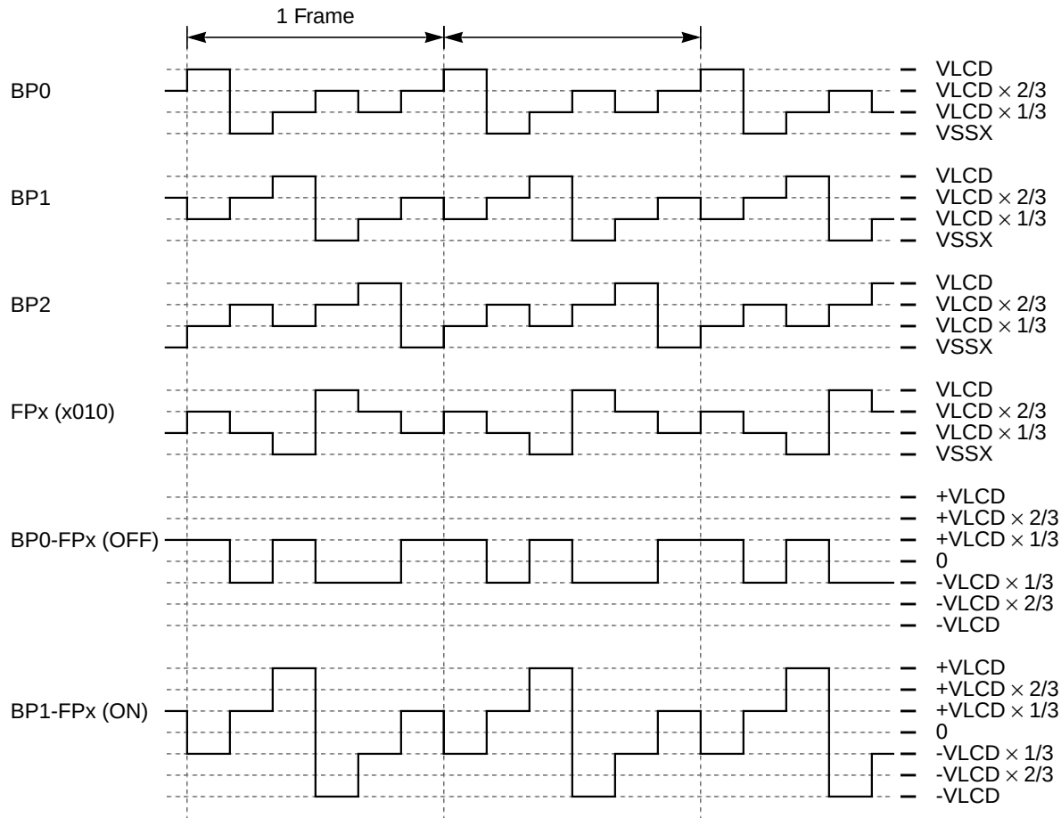
Figure 8-12. 1/3 Duty and 1/3 Bias
