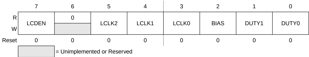
Figure 8-2. LCD Control Register 0 (LDCR0)
