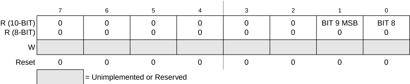
Figure 7-20. Right Justified, ATD Conversion Result Register x, High Byte (ATDDRxH)
