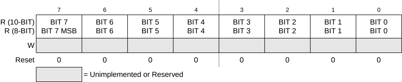
Figure 7-21. Right Justified, ATD Conversion Result Register x, Low Byte (ATDDRxL)
