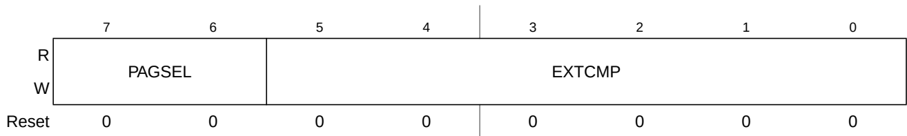
Figure 19-19. Debug Comparator B Extended Register (DBGCBX)
