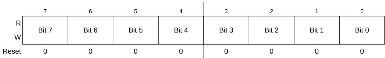
Figure 19-18. Debug Comparator A Register Low (DBGCAL)
