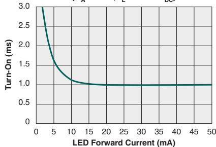
Typical Turn-On vs. LED Forward Current ( T_A=25^\circ\text{C} , I_L=120\text{mA}_{DC} )
