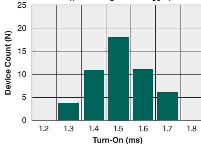
Typical Turn-On Time (N=50, T_A=25^\circ\text{C} , I_L=120\text{mA}_{DC} , I_F=5\text{mA} )
