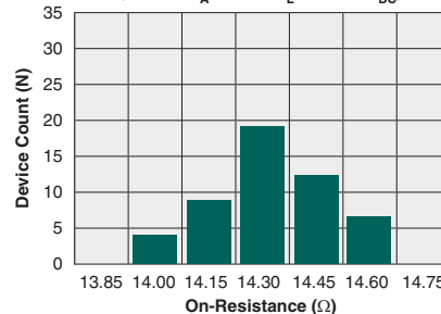
Typical On-Resistance Distribution (N=50, T_A=25^\circ\text{C} , I_L=120\text{mA}_{DC} )
