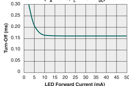
Typical Turn-Off vs. LED Forward Current ( T_A=25^\circ\text{C} , I_L=120\text{mA}_{DC} )
