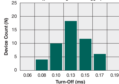
Typical Turn-Off Time (N=50, T_A=25^\circ\text{C} , I_L=120\text{mA}_{DC} , I_F=5\text{mA} )
