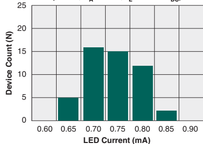
Typical I_F for Switch Operation (N=50, T_A=25^\circ\text{C} , I_L=120\text{mA}_{DC} )
