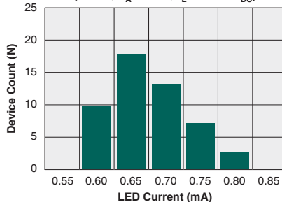
Typical I_F for Switch Dropout (N=50, T_A=25^\circ\text{C} , I_L=120\text{mA}_{DC} )
