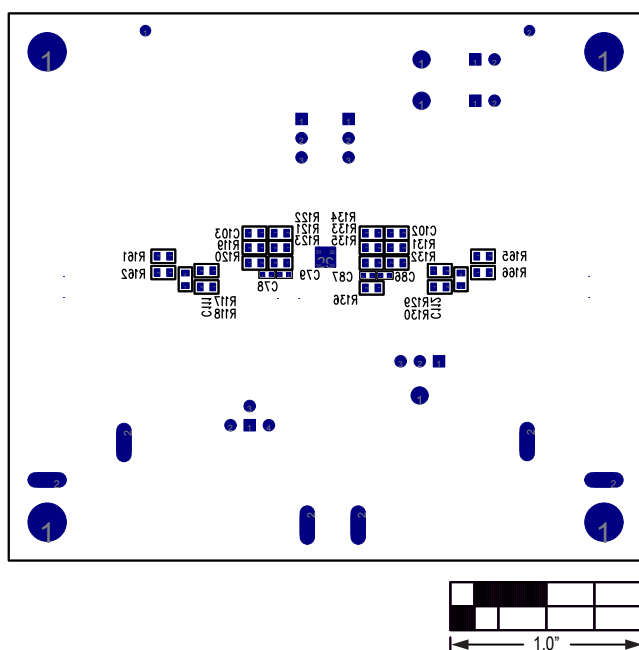
Figure 7. MAX16932 EV Kit Component Placement Guide—Solder Side
