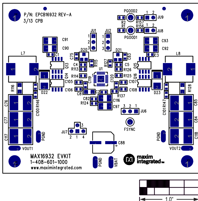
Figure 6. MAX16932 EV Kit PCB Layout—Solder Side
