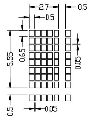
LED BKL
