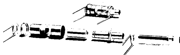
FORM FACTOR V, COLLARED BUSHING SEALED CONSTRUCTION
