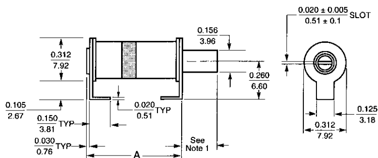
HORIZONTAL MOUNT
