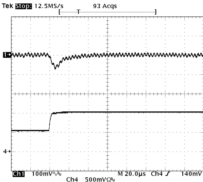
Fig-1.8V-6: Output voltage response for V_{out}=1.8V to positive load current step change from 5A to 10A with slew rate of 5A/us at V_{in}=12V . C_o=47\mu F \times 2 ceramic. Top trace: output voltage (100mV/div.) Bottom trace: load current (5A/div.) Time scale: 20us/div.
