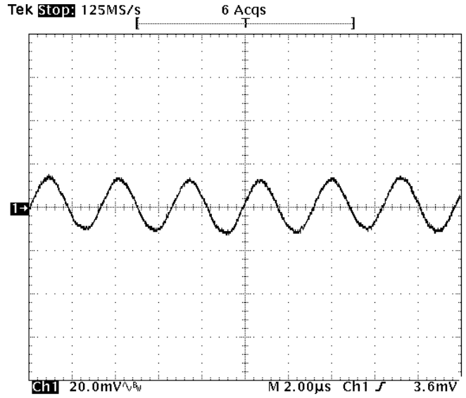
Fig-3.3V-5: Output voltage ripple (20mV/div.) for V_{out}=3.3V at full rated load current into a resistive load with external capacitance 47uFx2 ceramic + 1uF ceramic at V_{in}=12V . Time scale: 2 us/div
