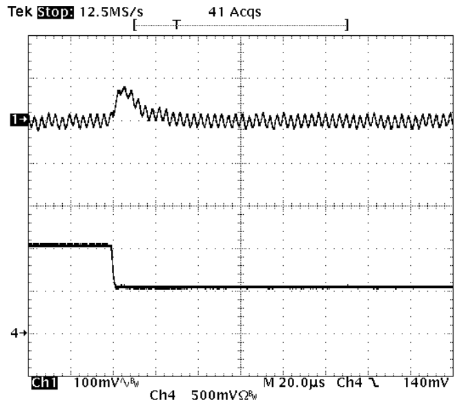
Fig-3.3V-7: Output voltage response for V_{out}=3.3V to negative load current step change from 10A to 5A with slew rate of -5A/us at V_{in}=12V . C_o=47uFx2 ceramic. Top trace: output voltage (100mV/div.) Bottom trace: load current (5A/div.) Time scale: 20us/div.
