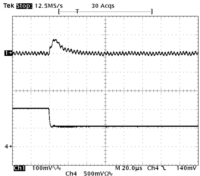
Fig-1.8V-7: Output voltage response for V_{out}=1.8V to negative load current step change from 10A to 5A with slew rate of -5A/us at V_{in}=12V . C_o=47\mu F \times 2 ceramic. Top trace: output voltage (100mV/div.) Bottom trace: load current (5A/div.) Time scale: 20us/div.
