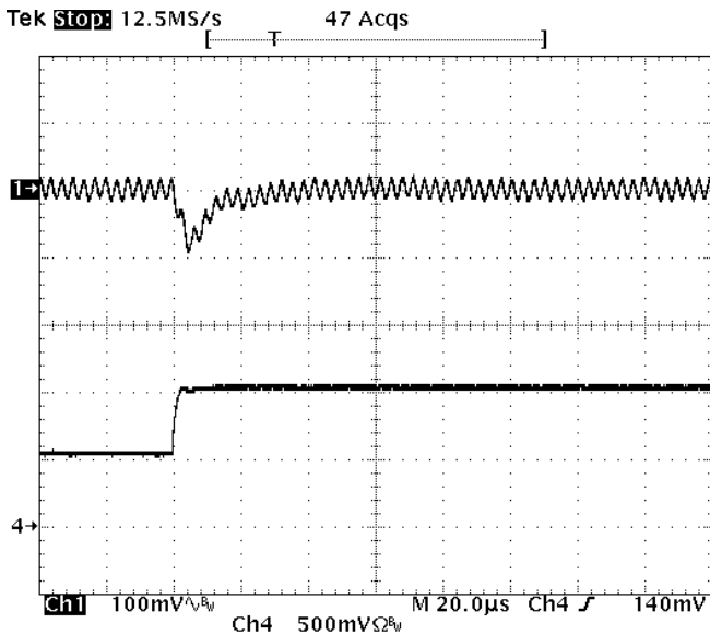
Fig-3.3V-6: Output voltage response for V_{out}=3.3V to positive load current step-change from 5A to 10A with slew rate of 5A/us at V_{in}=12V . C_o=47uFx2 ceramic. Top trace: output voltage (100mV/div.) Bottom trace: load current (5A/div.) Time scale: 20us/div.
