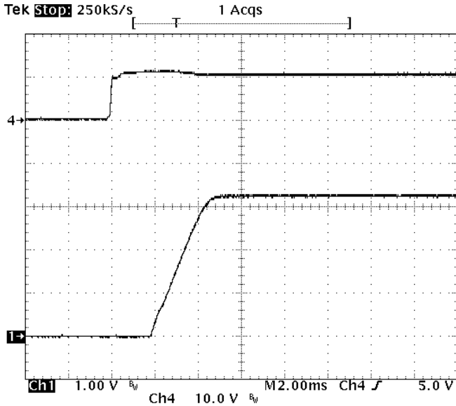
Fig-3.3V-4: Turn-on transient for V_{out}=3.3V with application of V_{in} at full rated load current (resistive) and 47uFx2 external capacitance at V_{in}=12V . Top trace: V_{in} (10V/div.) Bottom trace: output voltage (1V/div.) Time scale: 2ms/div.
