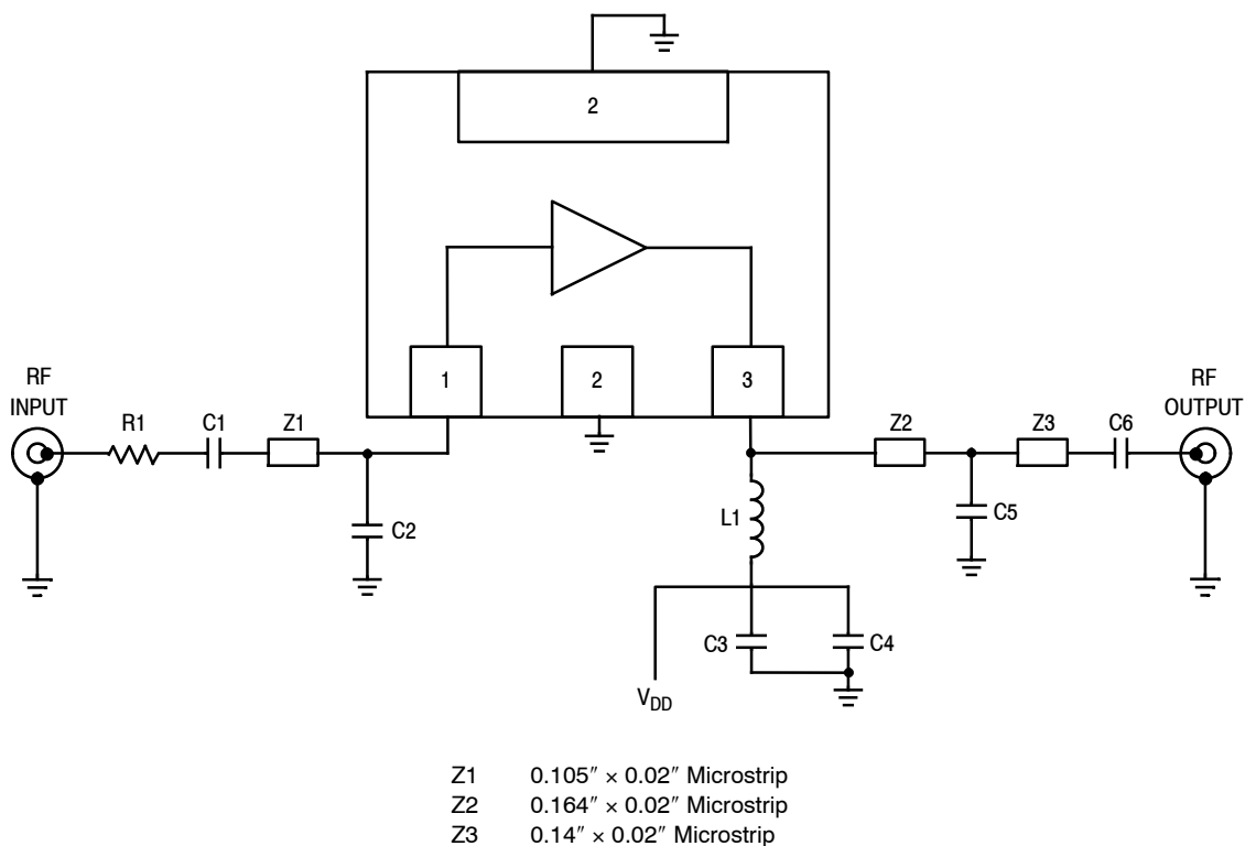
Figure 20. MMG30301BT1 Test Circuit Schematic
