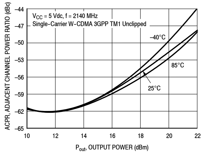
Figure 11. Single-Carrier W-CDMA Adjacent Channel Power Ratio versus Output Power and Temperature
