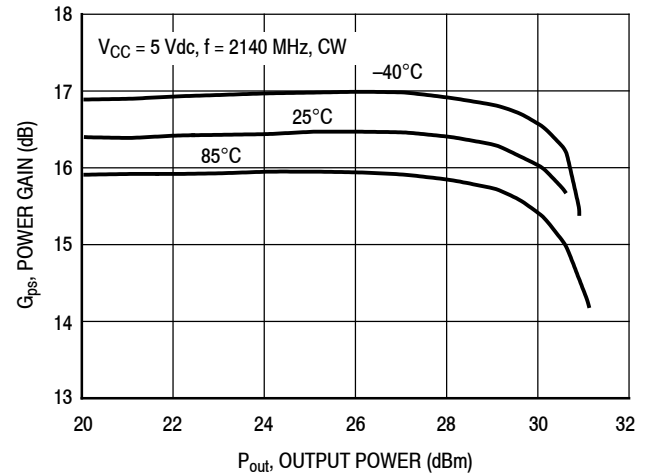
Figure 9. Power Gain versus Output Power and Temperature
