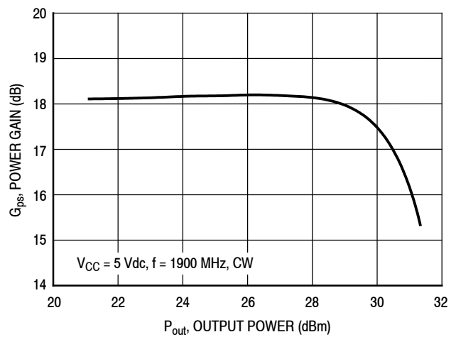
Figure 25. Power Gain versus Output Power
