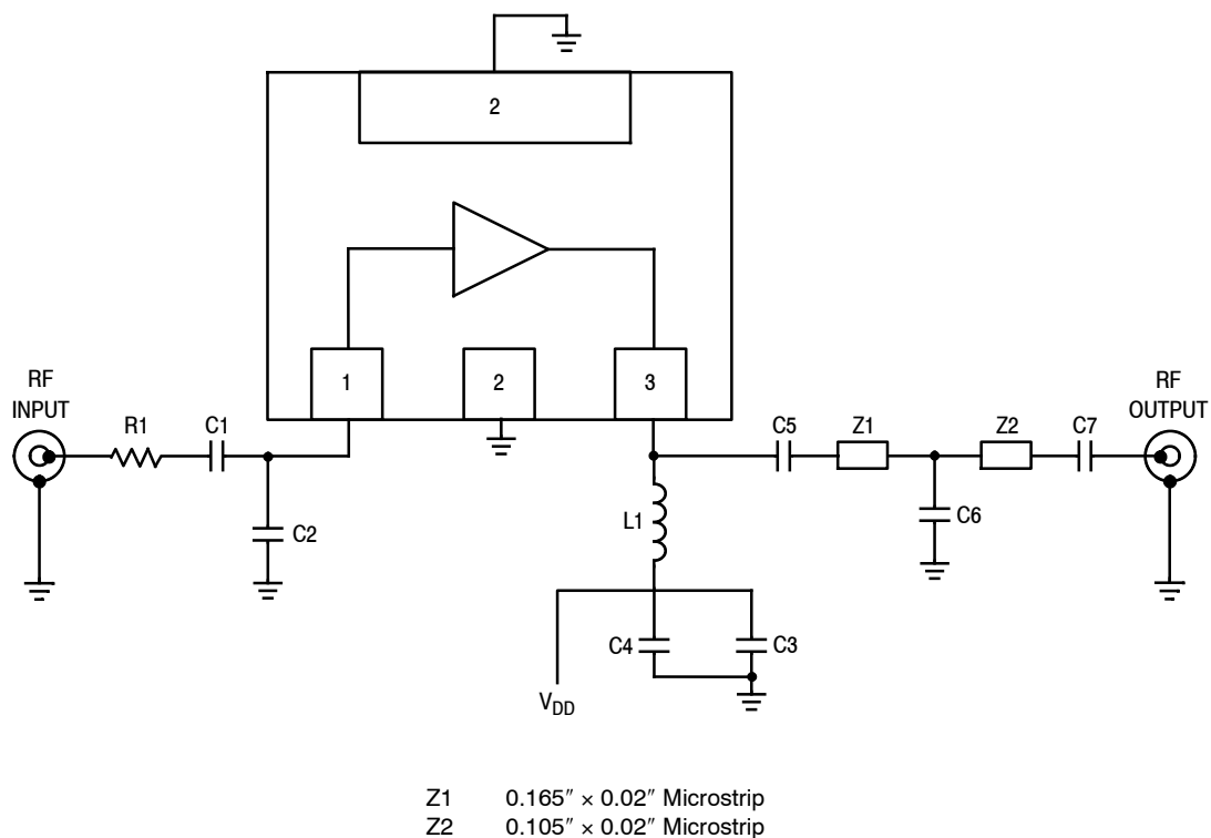
Figure 44. MMG30301BT1 Test Circuit Schematic
