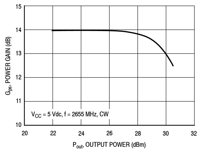
Figure 41. Power Gain versus Output Power
