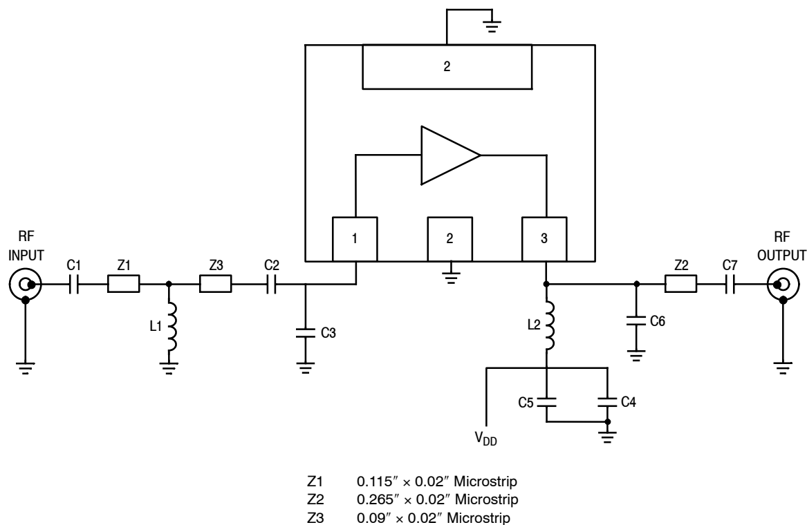
Figure 36. MMG30301BT1 Test Circuit Schematic
