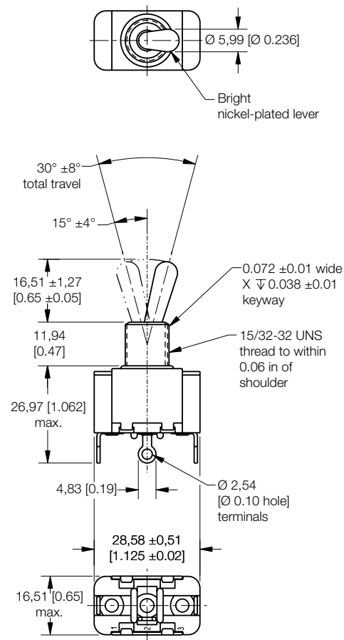
Figure 3. Single pole, standard lever, solder terminals
