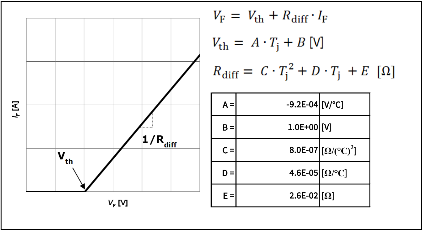
Figure 6 Simplified forward characteristics model V_F = f(I_F) ; -40^\circ\text{C} < T_j < 175^\circ\text{C} ; I_F < 32 \text{ A}
