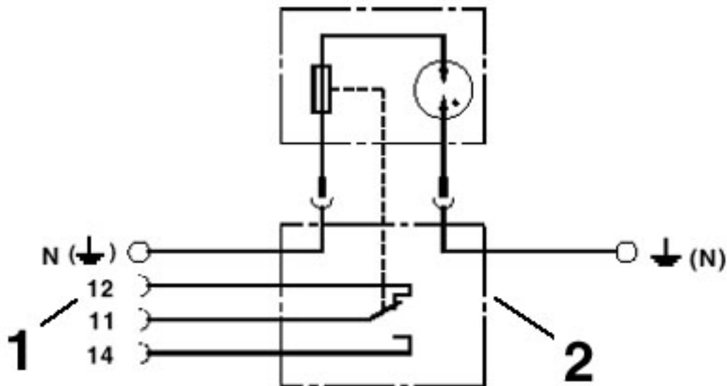
Circuit diagram
