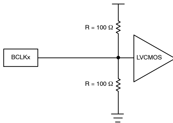
Figure 10. Optional Thevenin Termination
