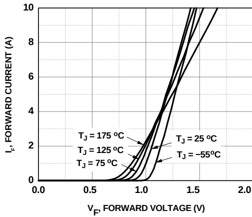
Figure 1. Forward Characteristics
