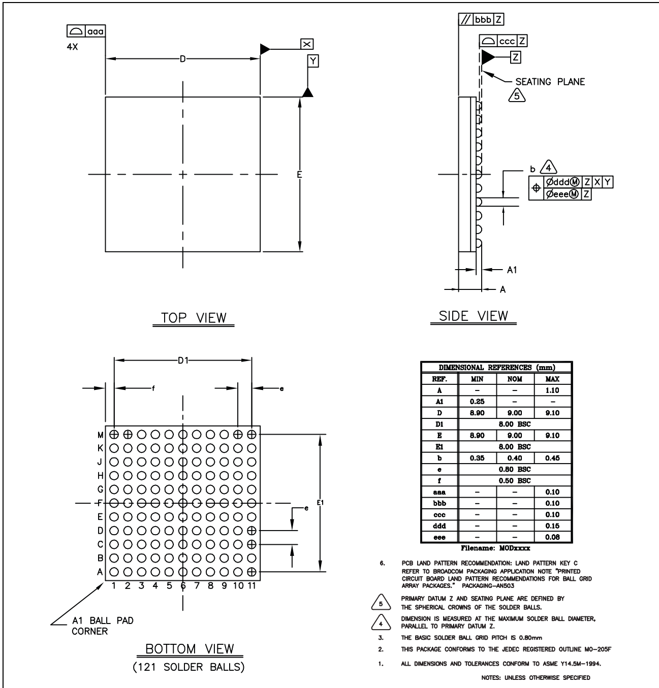
Figure 31. 121-Pin FBGA
