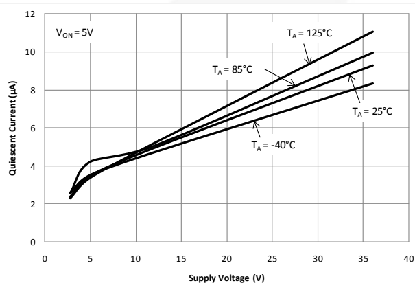
Figure 16. Quiescent Current vs. Supply Voltage (OFF)
