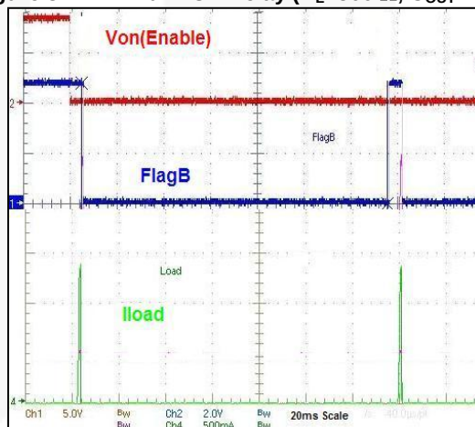
Figure 33. 12V Restart Time (Switch Turned ON into Persistent Over-Current Condition, t_{RESTART}=127.5\text{ ms} )
