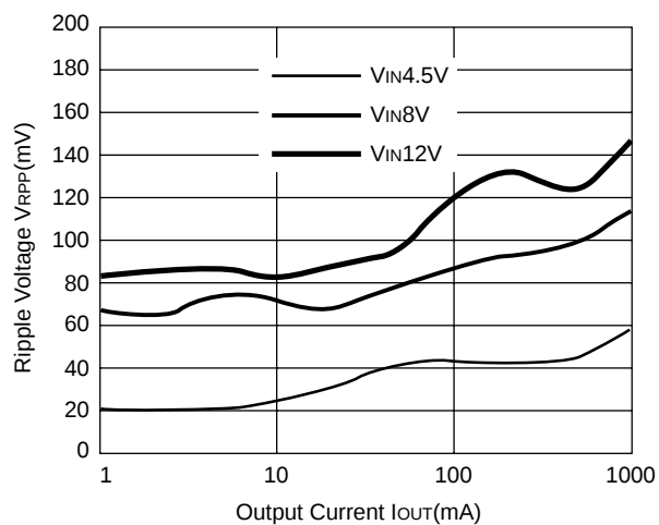
R1223N332A L=27 \mu H
