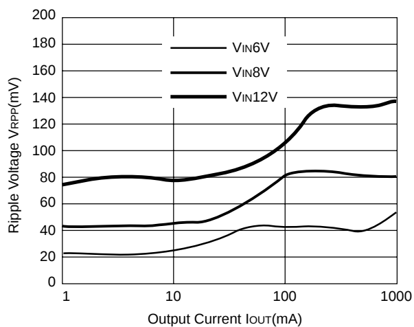
R1223N502A L=27 \mu H
