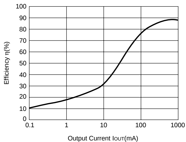
R1223N502C( V_{IN}=12V ) CD104-27 \mu H Si3443DV
