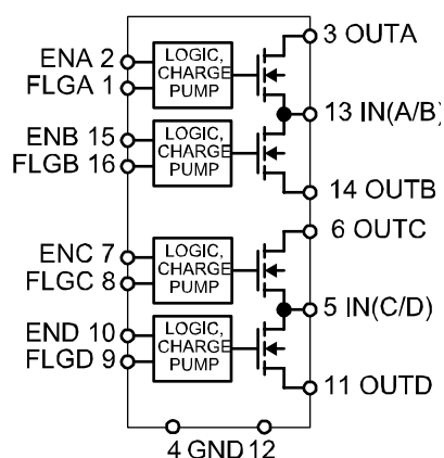
Functional Pinout
