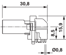
M12 flush-type male connector, angled
