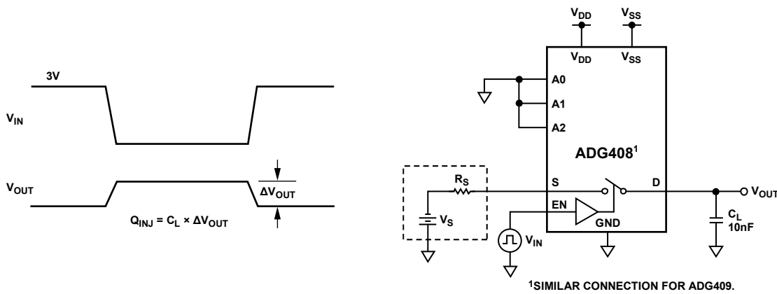
Figure 25. Charge Injection
