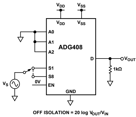
Figure 26. Off Isolation
