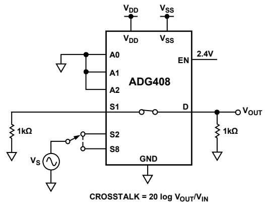
Figure 27. Channel-to-Channel Crosstalk
