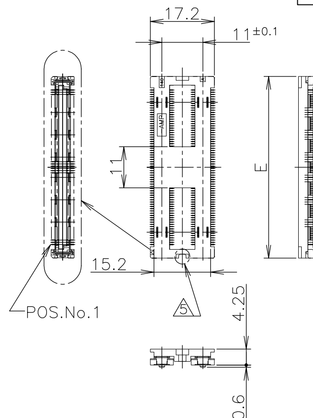
CONNECTOR DETAIL
