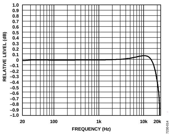
Figure 13. Relative Level vs. Frequency at -10 dBFS Normalized, 32x Decimation, f_s = 48 kHz
