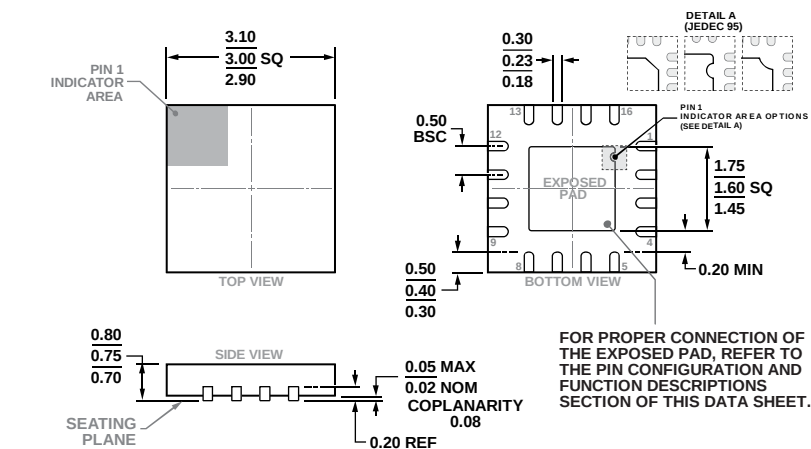
Figure 27. 16-Lead Lead Frame Chip Scale Package [LFCSP] 3 mm × 3 mm Body and 0.75 mm Height (CP-16-22) Dimensions shown in millimeters
