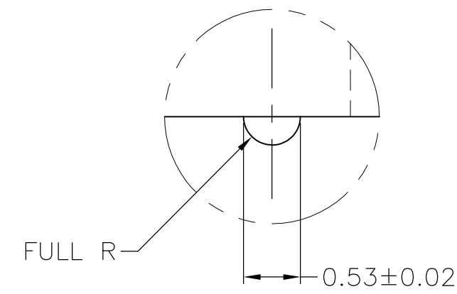
DETAIL Z SCALE 20:1
