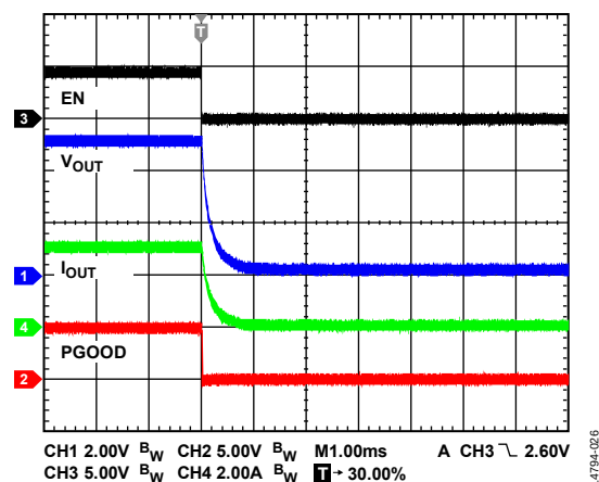
Figure 26. Shutdown with Full Load
