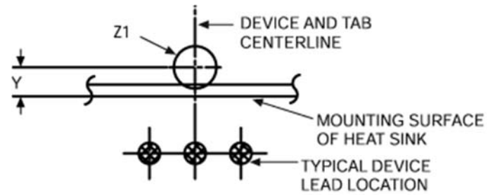
Mounting Details:
