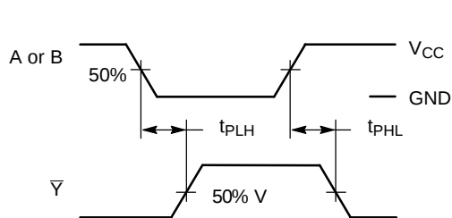
Figure 4. Switching Waveforms
