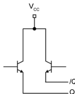
Figure 2b. Simplified LVPECL Output Stage
