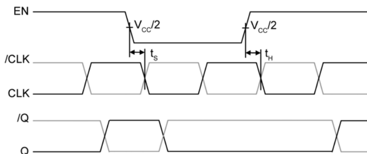
t_{PD} – Set-Up and Hold Time EN -to-Differential Out
