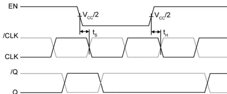
t_{PD} – Set-Up and Hold Time \text{EN} -to-Differential Out
