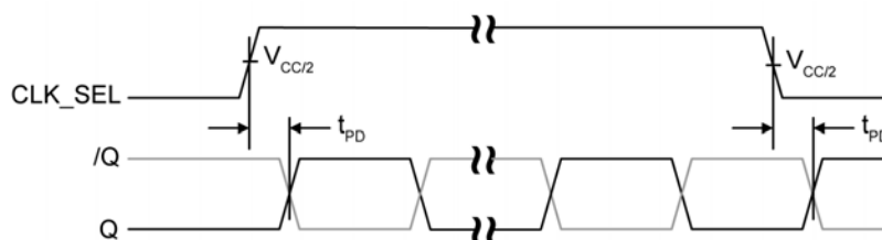
t_{PD} – \text{CLK\_SEL} -to-Differential Out
