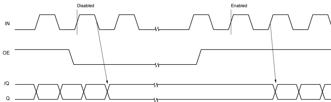
Figure 1c. Enable Output Timing Diagram
