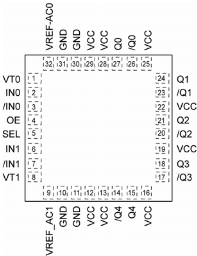
32-Pin MLF ® (MLF-32)
