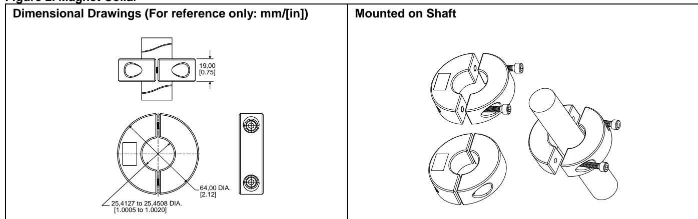
Figure 2. Magnet Collar
