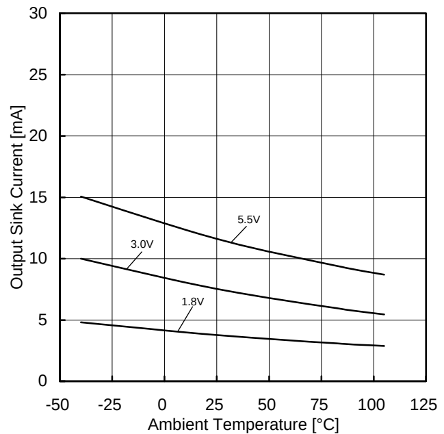
Figure 30. Output Sink Current vs Ambient Temperature (OUT=VSS+0.4V)
