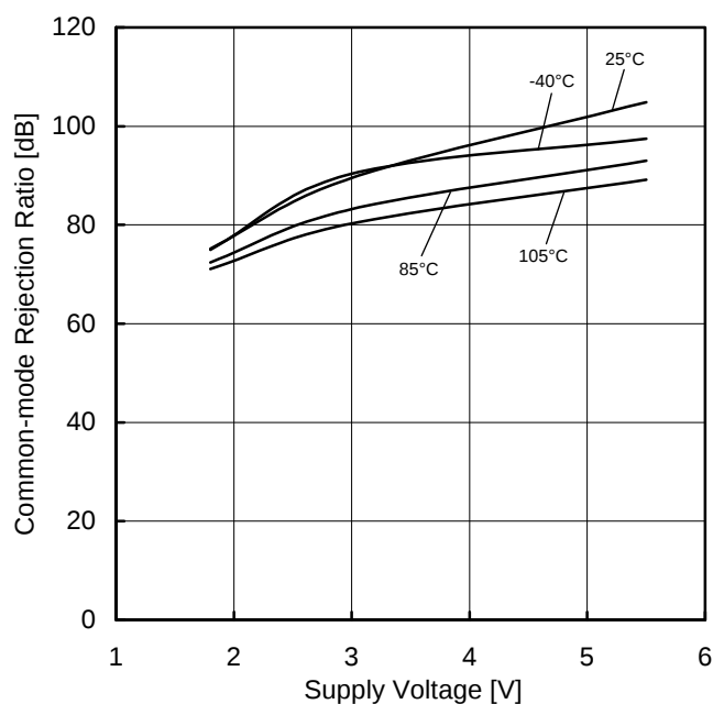
Figure 36. Common-mode Rejection Ratio vs Supply Voltage
