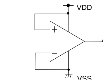
Figure 45. Example of Application Circuit for Unused Comparator
