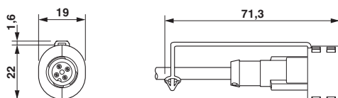
EXCLIP mounted socket
