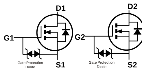
Equivalent Circuit
