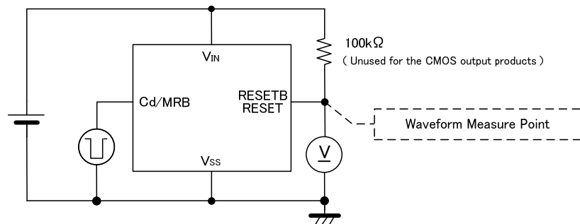
CIRCUIT⑦
