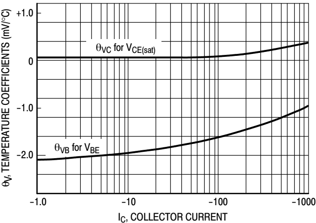
Figure 15. Temperature Coefficients
