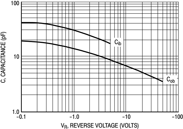
Figure 16. Capacitances
