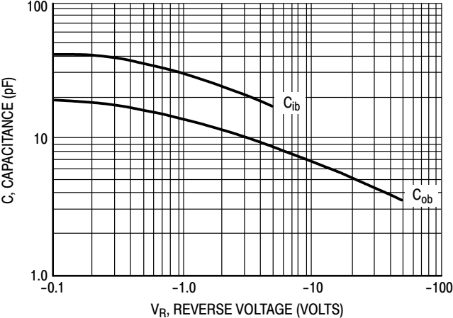
Figure 16. Capacitances
