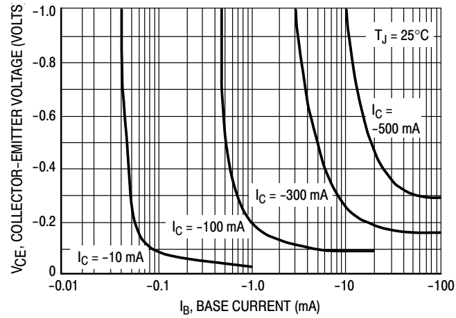
Figure 6. Saturation Region
