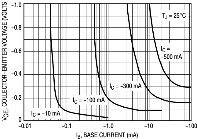
Figure 14. Saturation Region
