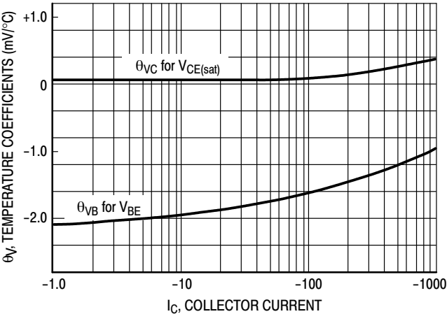
Figure 7. Temperature Coefficients
